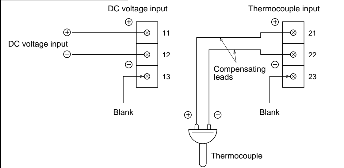
Example Input terminal wiring
