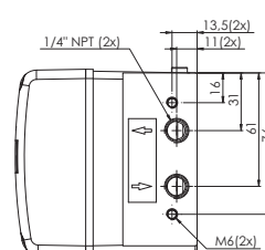
S09 "Double D Spindle"
