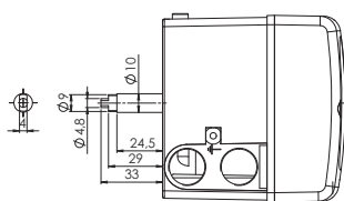
S23 "Namur Spindle"
