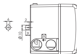
S09 "Double D Spindle"
