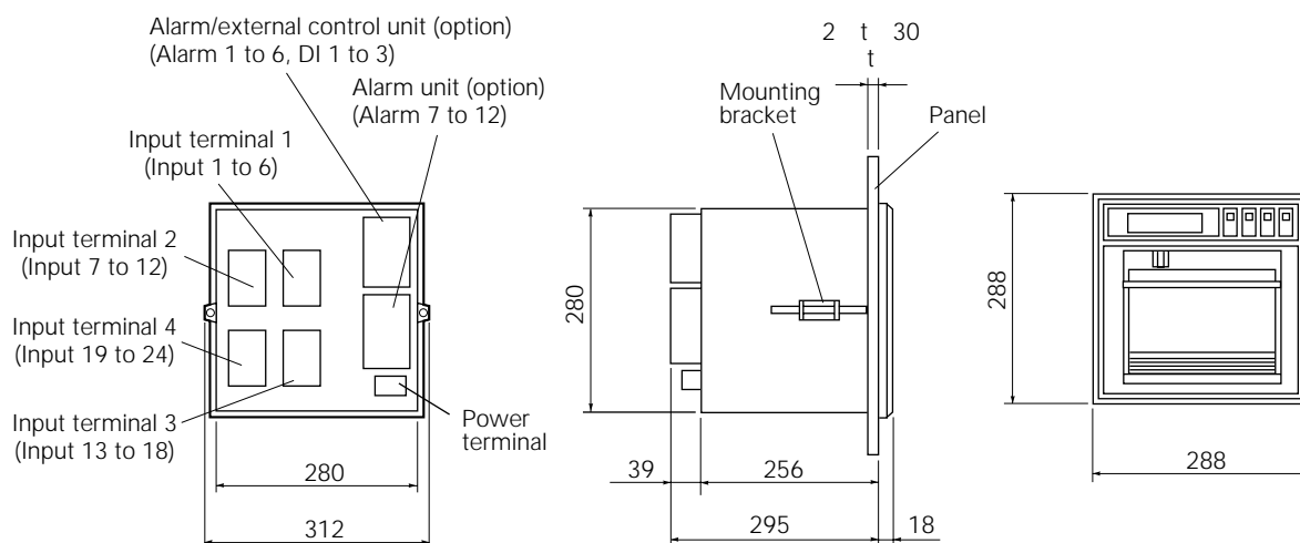
Panel cutout
