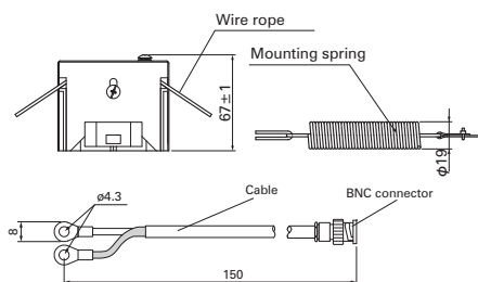
Signal cable conversion cord (accessories)
