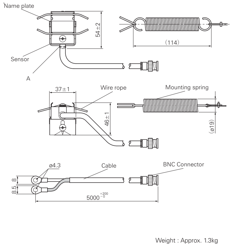
Detector FSD41 (Middle type)
