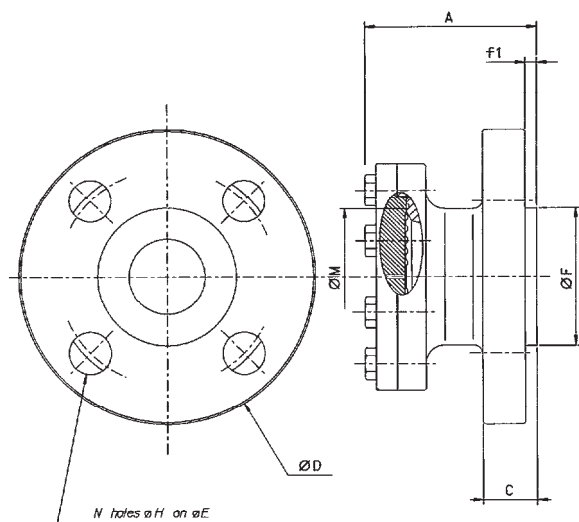
FLANGES DIMENSIONS
